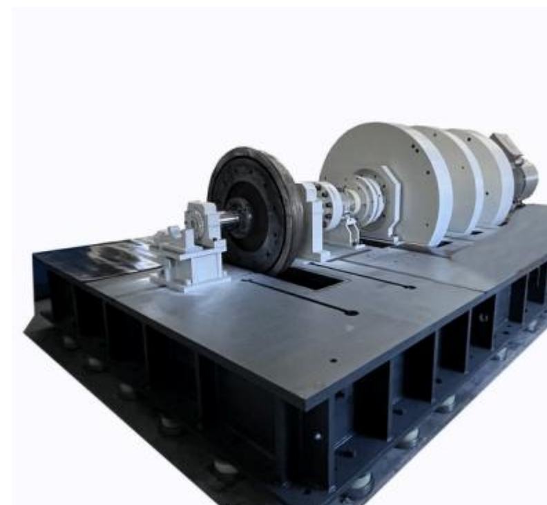
Large Inertia High-Speed Tester
